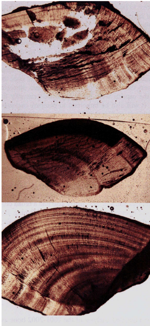
Fig. 7. Typical problems interpreting the sectioned sea catfish otoliths. Top – cracked otolith; Middle – burnt otolith; Bottom – otolith from mature individual. (Photographs by Mark Beech and Mohsen al-Husaini).
