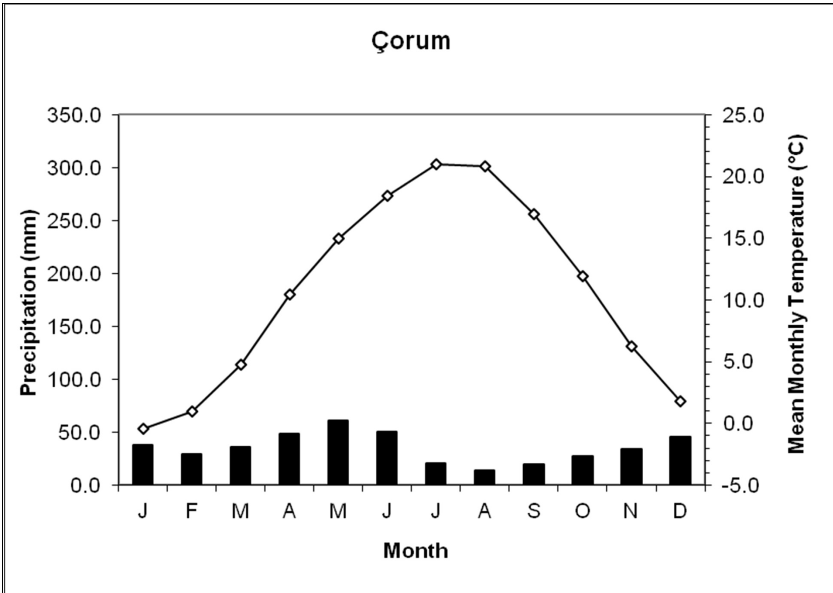
Figure 2.1. Precipitation and temperature data for Çorum (average for 1930-2000).
