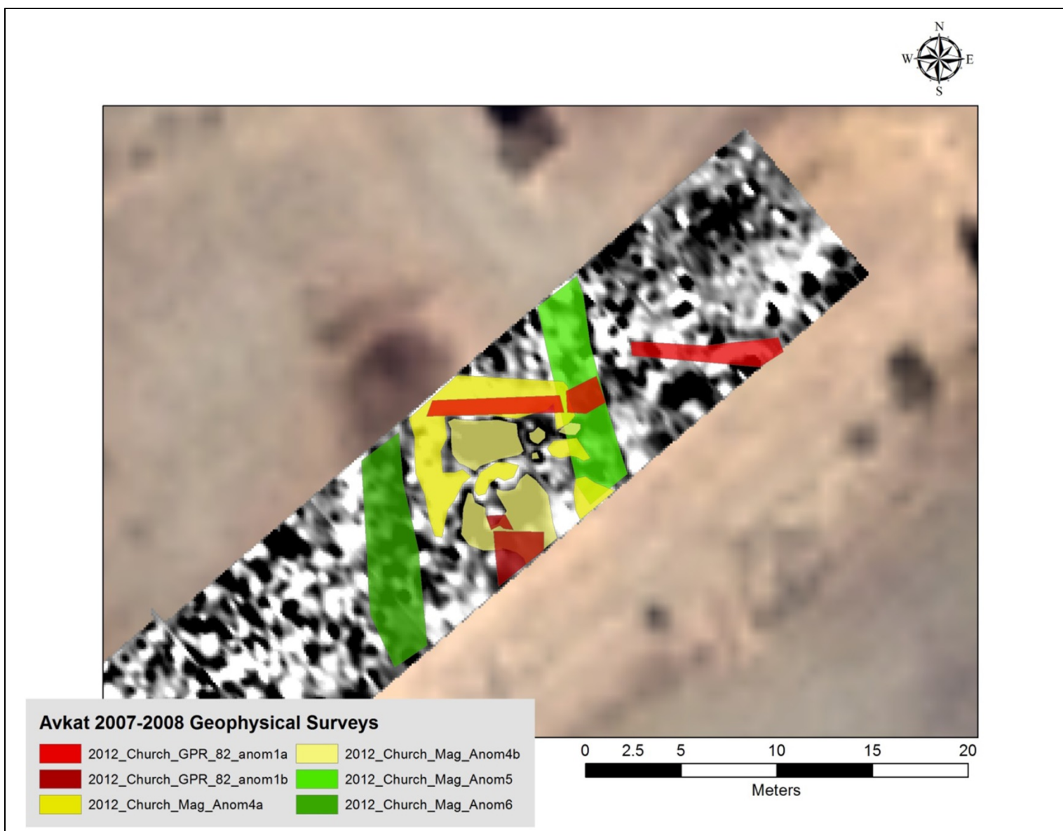
Map A1.10. North - south running anomalies (green) that bound the strong magnetic structure anomaly.
