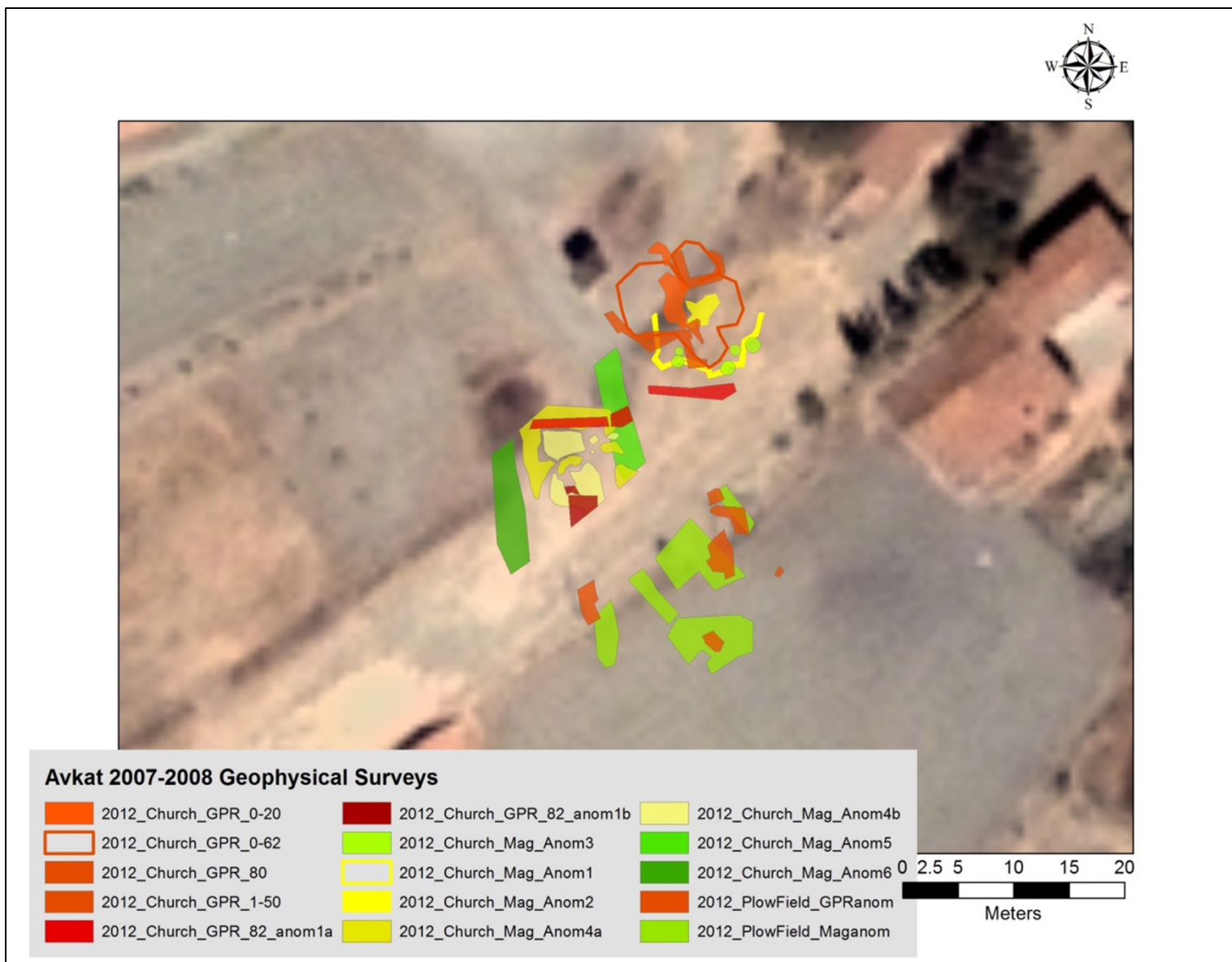
Map A1.12. Interpretations for the GPR and magnetic gradient surveys in the 'Church' survey area.
