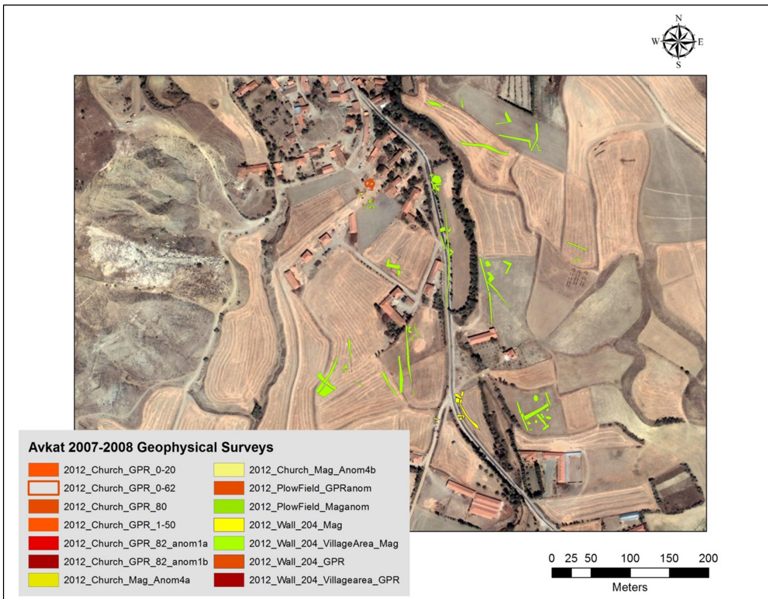
Map A1.15. GPR and magnetic gradient interpretations for F0204.
