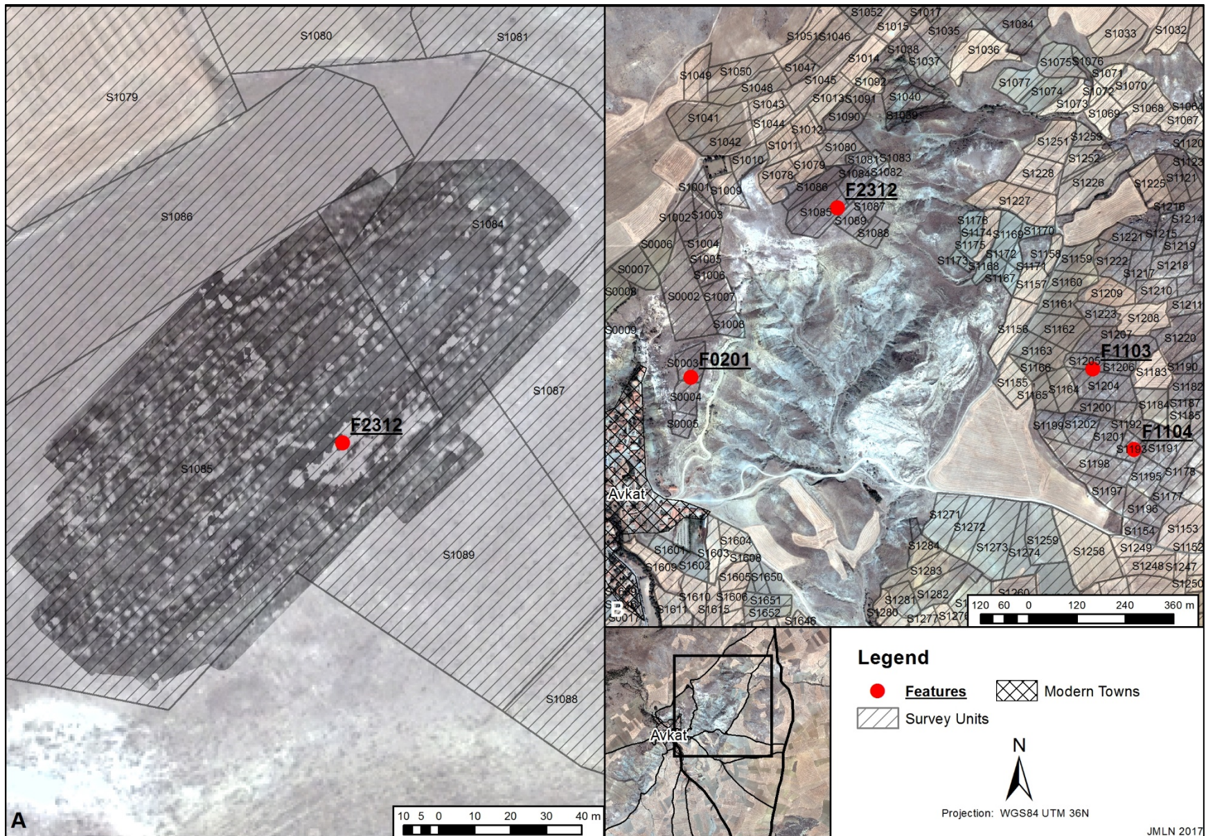
Map 7.5. Magnetometry of Kabak Tepesi (a) and locations of defensive features east of Avkat (b).
