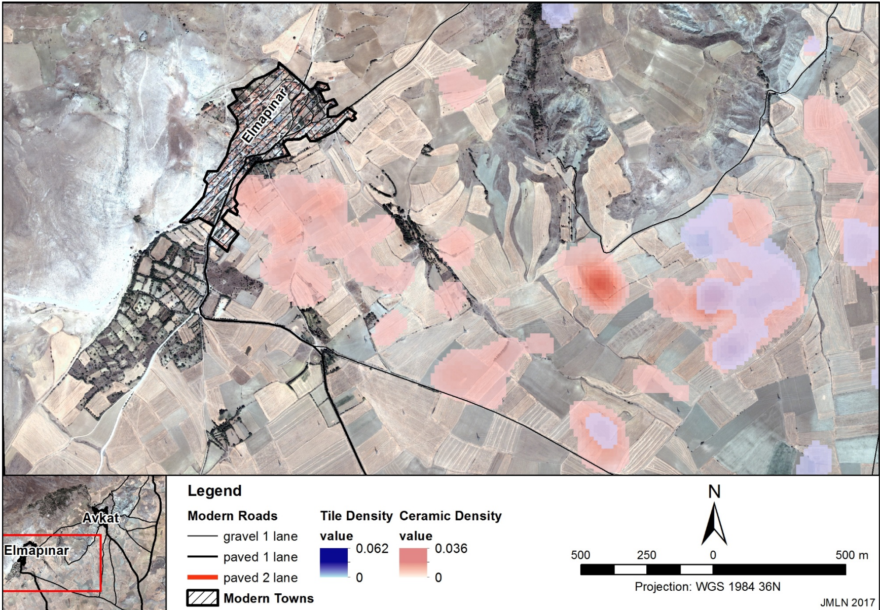
Map 7.7. Map of densities of ceramics and tile around Elmapinar.
