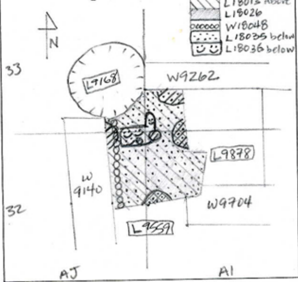
Sketch plan 1:100
